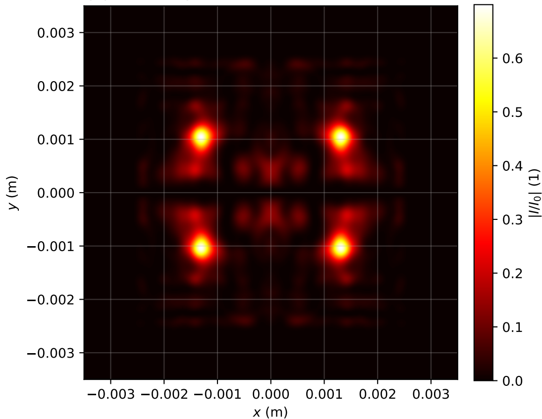
Intensity profile I(x, y, z = 3.742)/I_0 , P_{in}=8.0P_{cr} , artificial time
